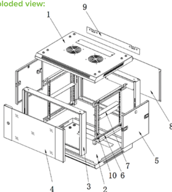
Exploded view:
