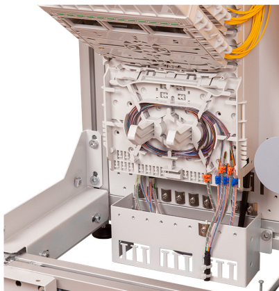
MDO Subrack
