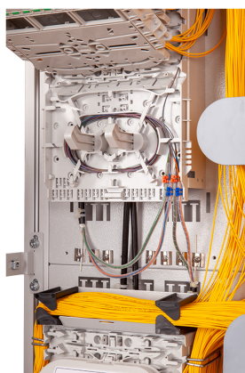
MDO Subrack
