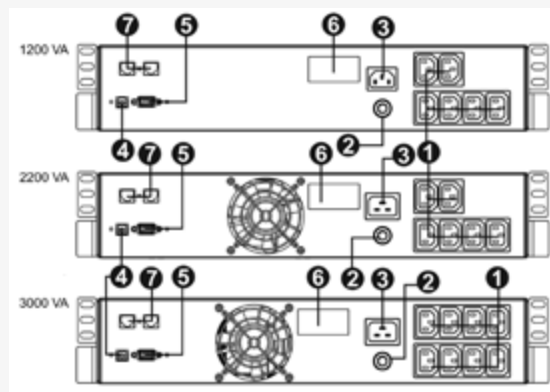
Above: rear view of Compact RM 1200, 2200, 3000 VA
