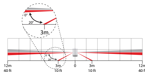
Range Adjustment
